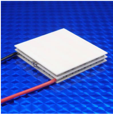
2 Stage TEC
