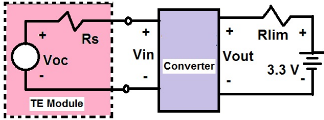
Figure 3 –Measurement Set-up for Performance Curves
