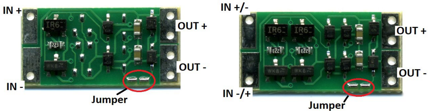
Figure 2 – Reverse Side of ELC-UBV120 and ELC-BVB120
