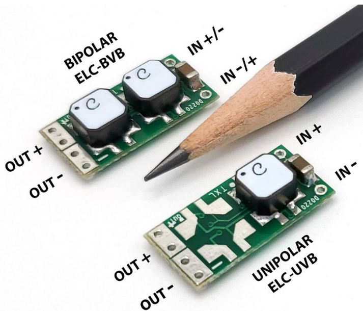
Figure 1 – Input and Output Polarity for Unipolar and Bipolar Versions
