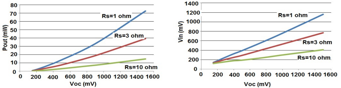
Figure 4 – Performance Curves for Power Delivery to a 3.3V Lithium Ion Cell
