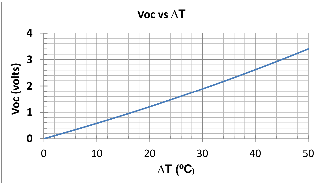
Figure 1 – Open Circuit (No Load) Voltage vs \Delta T for the TXL-127-03L
