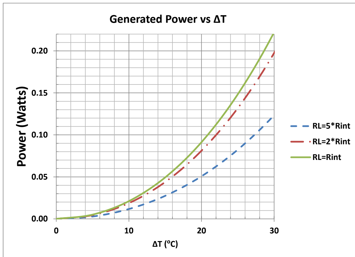
Figure 4 – Load Power as a Function of \Delta T for Three Different Load Resistances Using a TXL-127-03L Module
