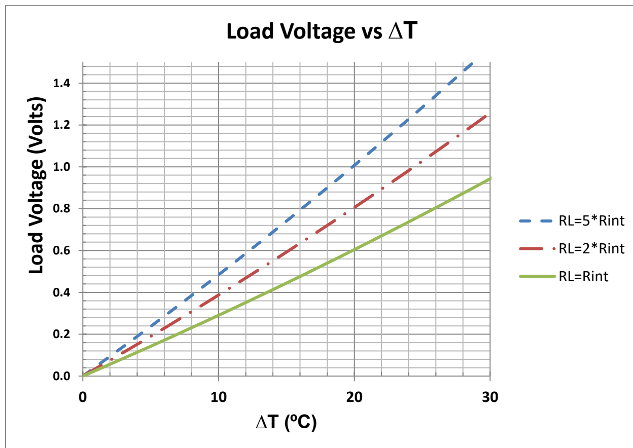
Figure 3 – Load Voltage as a Function of \Delta T for Three Different Values of Load Resistance for the TXL-127-03L
