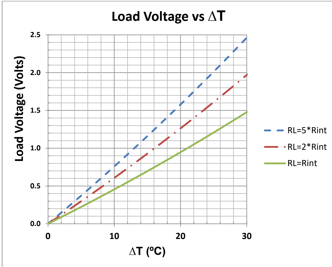
Figure 3 – Load Voltage as a Function of \Delta T for Three Different Values of Load Resistance for the TXL-199-02Q
