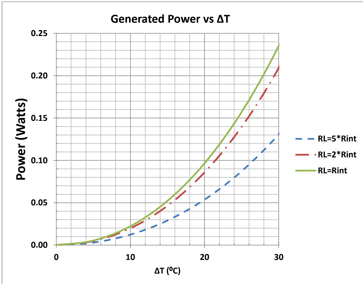
Figure 4 – Load Power as a Function of \Delta T for Three Different Load Resistances Using a TXL-199-02Q Module
