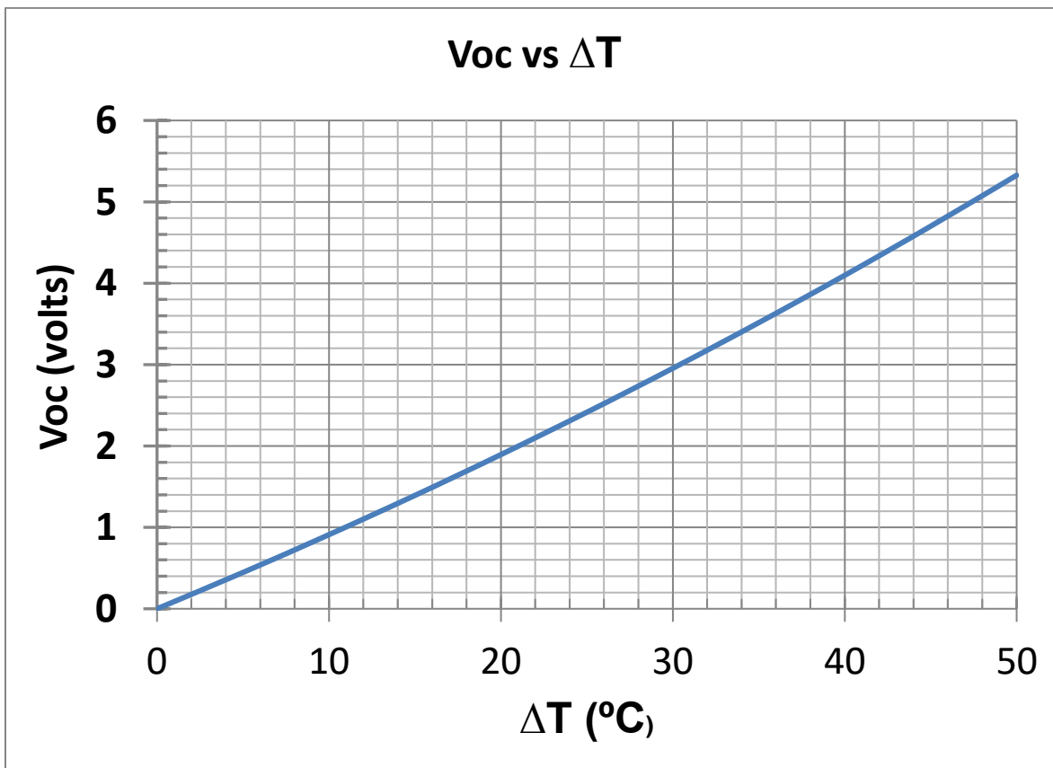
Figure 1 – Open Circuit (No Load) Voltage vs \Delta T for the TXL-199-02Q
