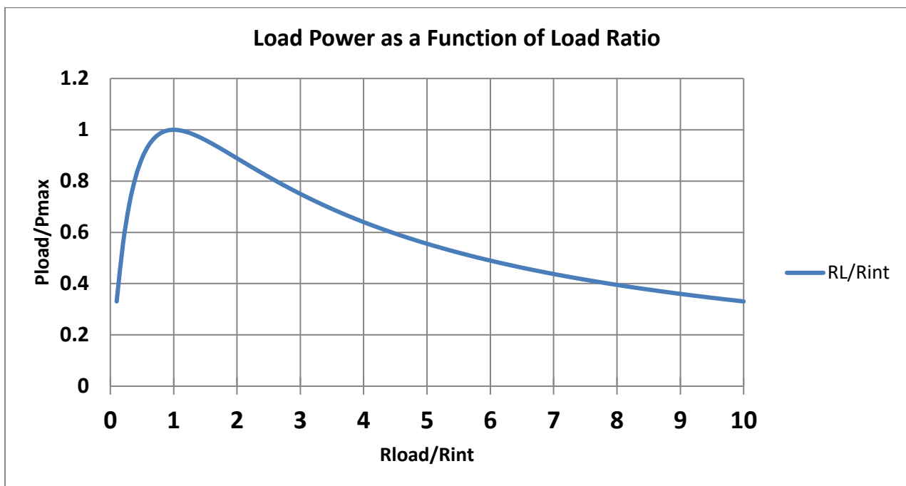
Figure 2 – Output Power as a Function of Load Resistance
