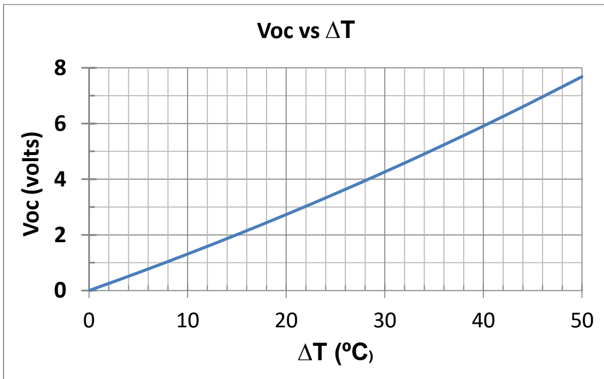
Figure 1 – Open Circuit (No Load) Voltage vs \Delta T for the TXL-287-03Z
