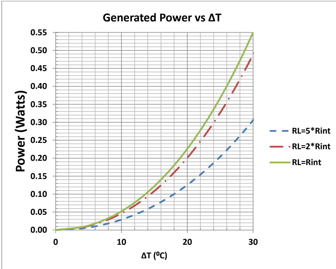
Figure 4 – Load Power as a Function of \Delta T for Three Different Load Resistances Using a TXL-287-03Z Module
