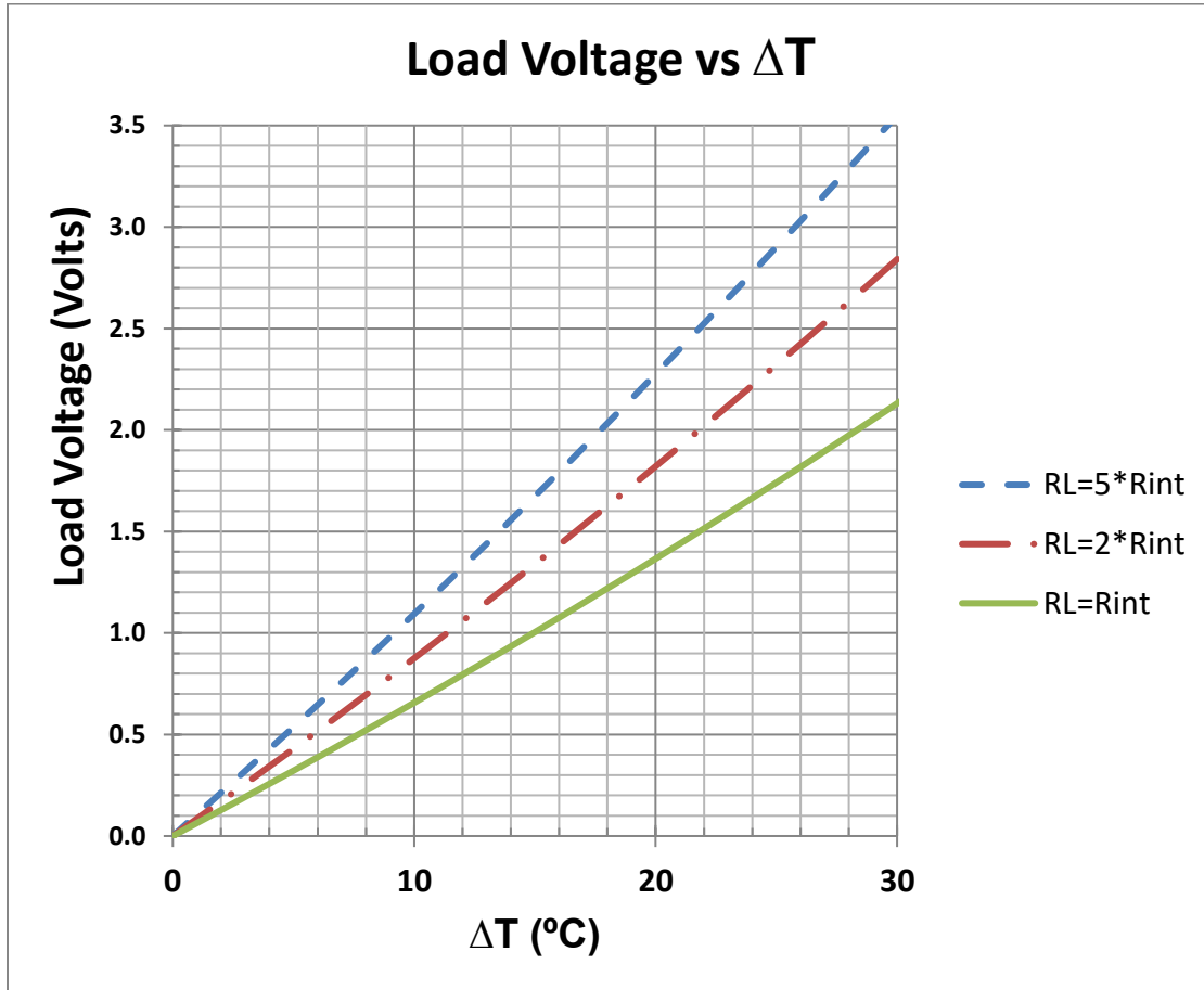
Figure 3 – Load Voltage as a Function of \Delta T for Three Different Values of Load Resistance for the TXL-287-03Z
